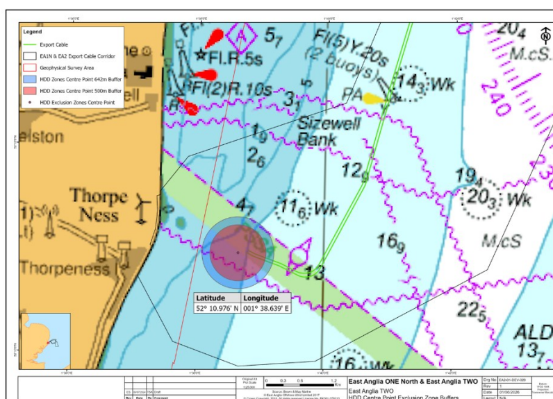
Figure 1: EA1N and EA2 Wind Farm Marine Works Location and JUB exclusion zone
