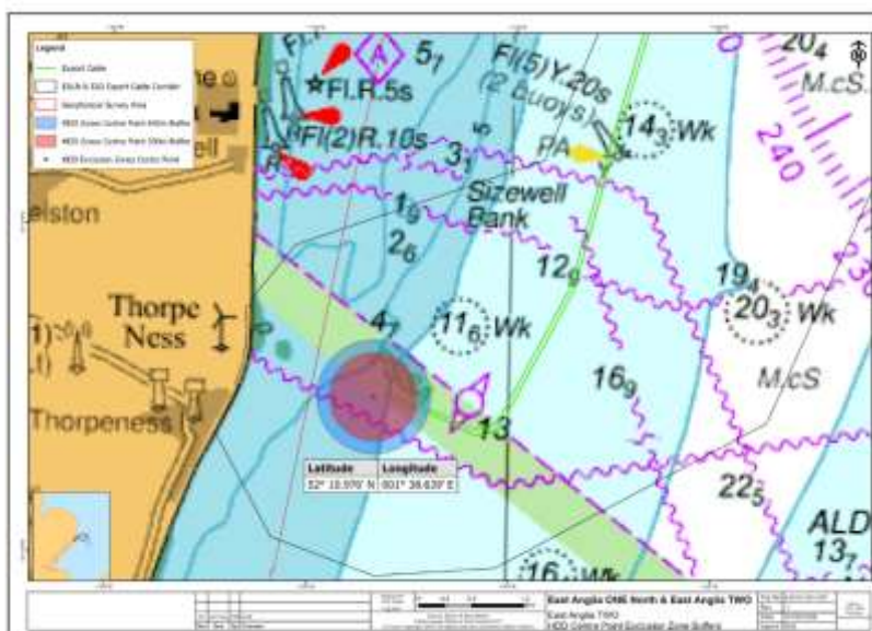
Figure 1: EA1N and EA2 Wind Farm Marine Works Location and JUB exclusion zone
